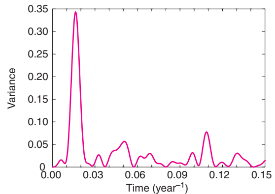
Figure 4. The truncated Fourier power spectrum of the reduced quadratic residuals.
