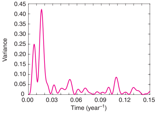
Figure 2. The truncated Fourier power spectrum of the straight-line residuals. We discarded frequencies between 0.15 and 0.5 \text{ yr}^{-1} to expand the low frequencies.
