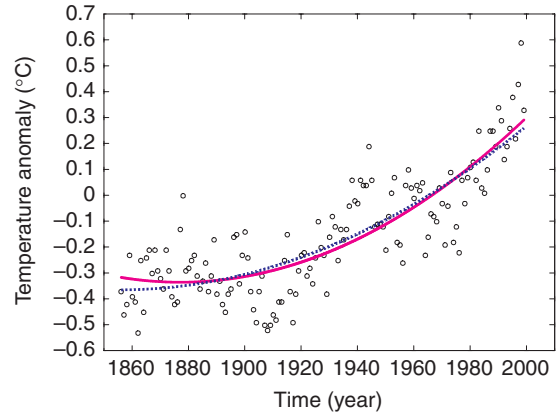
Figure 3. Quadratic and reduced quadratic fits to the global yearly average temperature anomalies. The solid curve is the full quadratic, and the dashed curve is the reduced quadratic (Equation 33).
