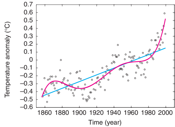
Figure 1. The straight line and fifth-degree polynomial fits to global yearly average temperature data. The plotted circles are temperature anomalies obtained by subtracting the mean temperature ( 14^\circ \text{C} ) for the years 1961 to 1990 from the actual measured averages.
