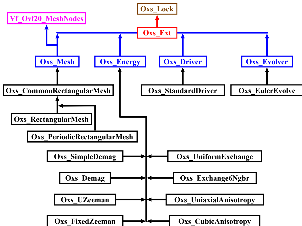
Figure 5.2: Oxs_Ext primary hierarchy class diagram.
