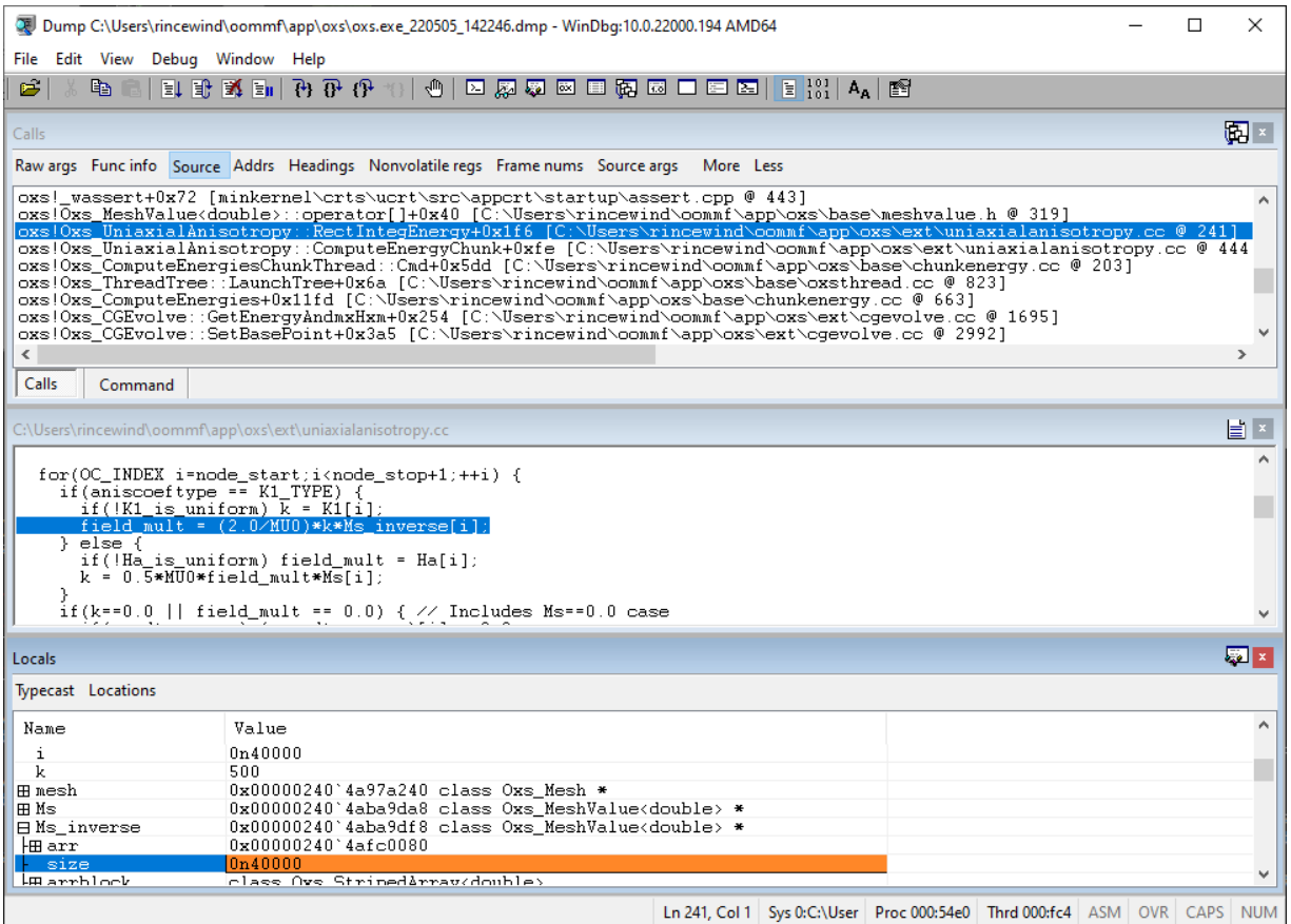
Figure 6.2: WinDbg screenshot displaying call stack, source code, and local variables read from a crash dump generated by procdump .
