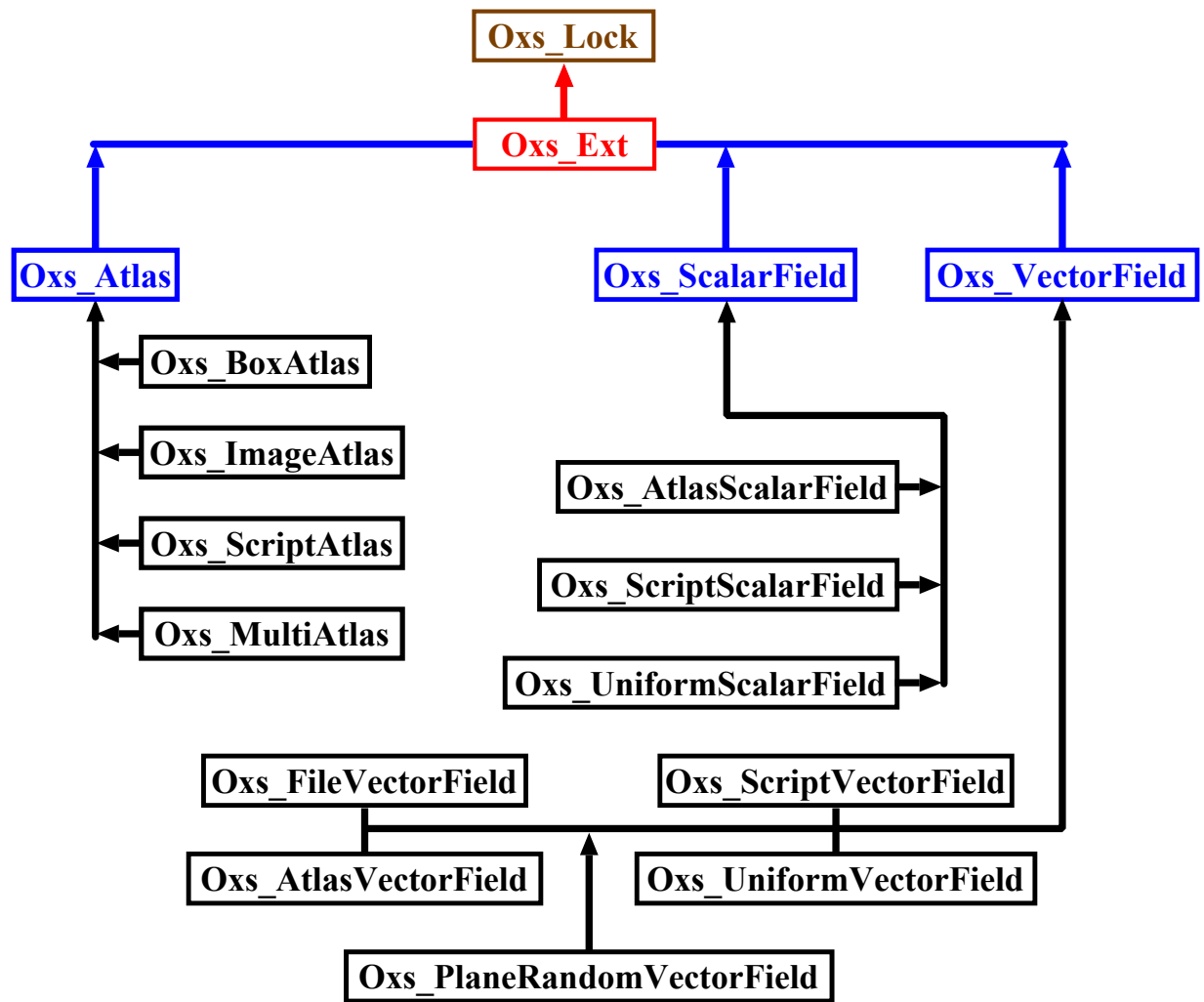
Figure 5.3: Oxs_Ext supplemental hierarchy class diagram.
