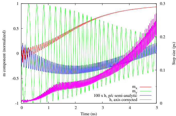
FIG. 2: Comparison of effectiveness of adjustable time step determination applied to the original semi-analytic predictor-corrector solver, and to the proposed axis-corrected alternative. Magnetization components m_x and m_y as a function of time are plotted against the scale on the left. Time step lengths as a function of time are plotted against the scale on the right. Note the scaling of the third curve for sake of visibility makes values appear one hundred times greater than they are.
