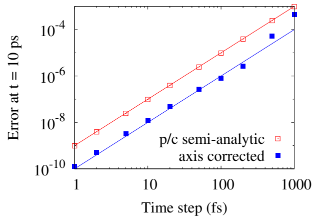
FIG. 1: Comparison of relative error vs time step length for the original semi-analytic predictor-corrector solver, and the proposed axis-corrected alternative.
